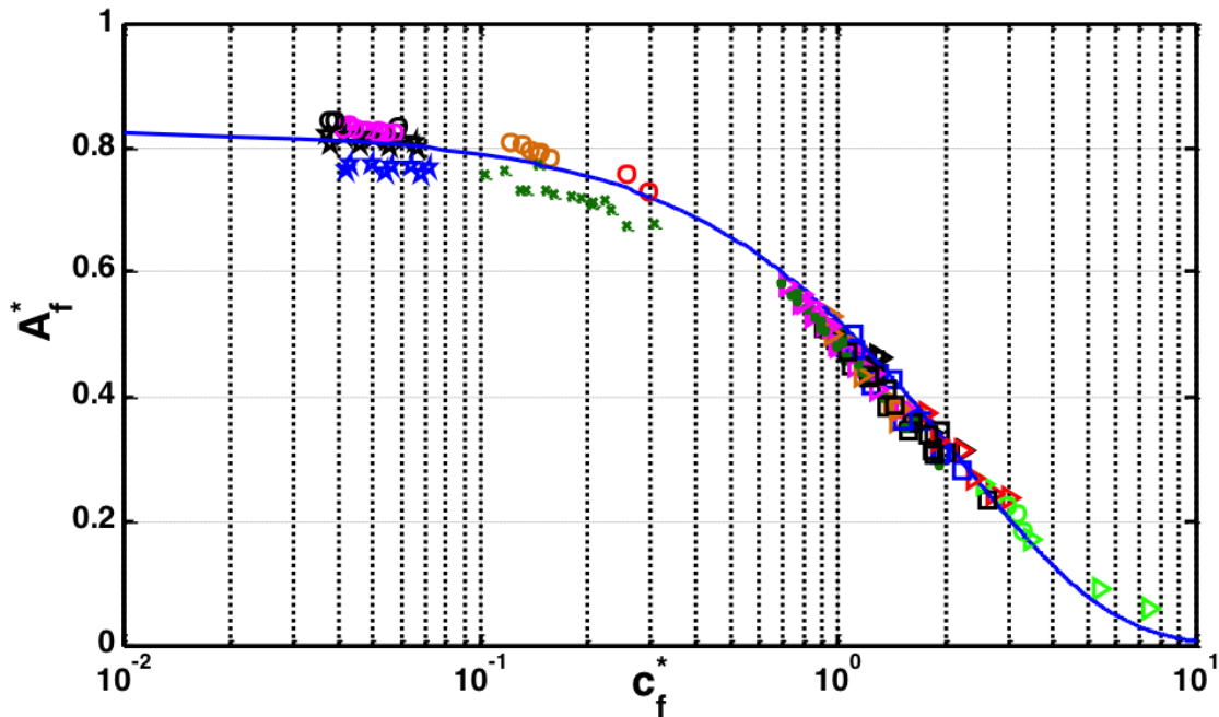
Figure H-1: A^* versus c_f^* for a wide range of top tension, SCR and lazy wave risers with and without stakes.
