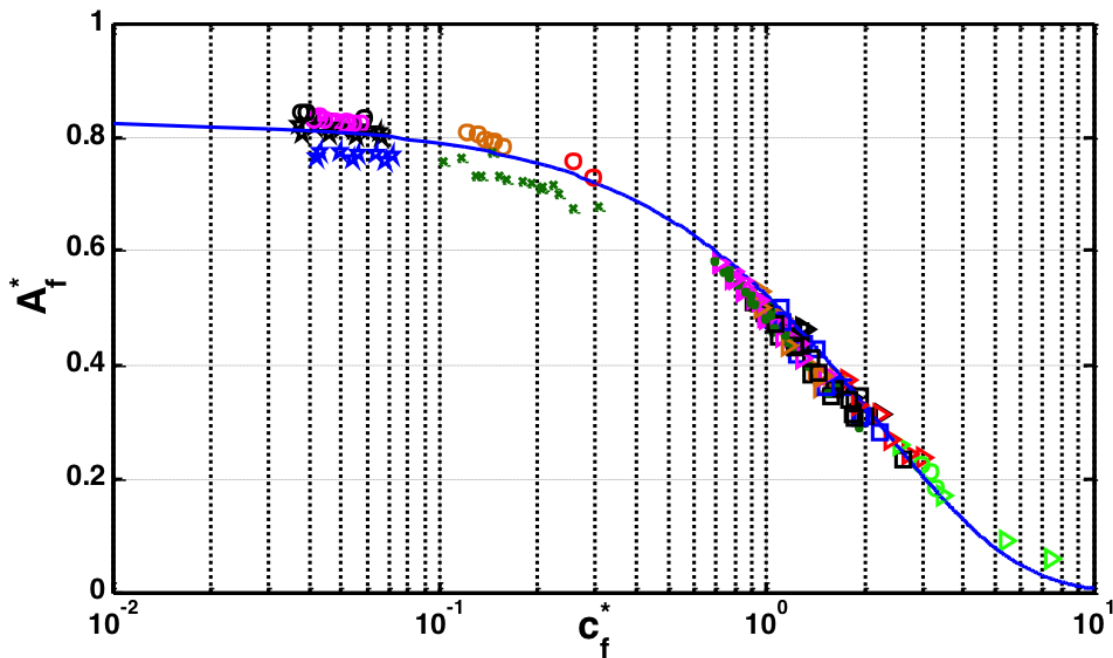
Figure H-1: A^* versus c^* for a wide range of top tension, SCR and lazy wave risers with and without stakes.
