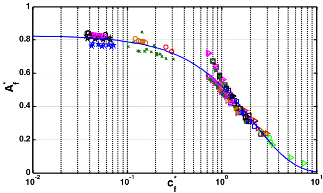
Figure H-2: A^* versus c^* for a wide range of top tension, SCR and lazy wave risers with and without strakes. The branch on the top side of the curve revealed a program bug during development testing that was subsequently resolved prior to release.
