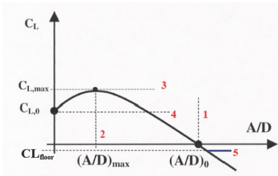
Figure B-1: SHEAR7 defines a smoothed lift coefficient curve by fitting two parabolas to three defined by four user-specified values.
