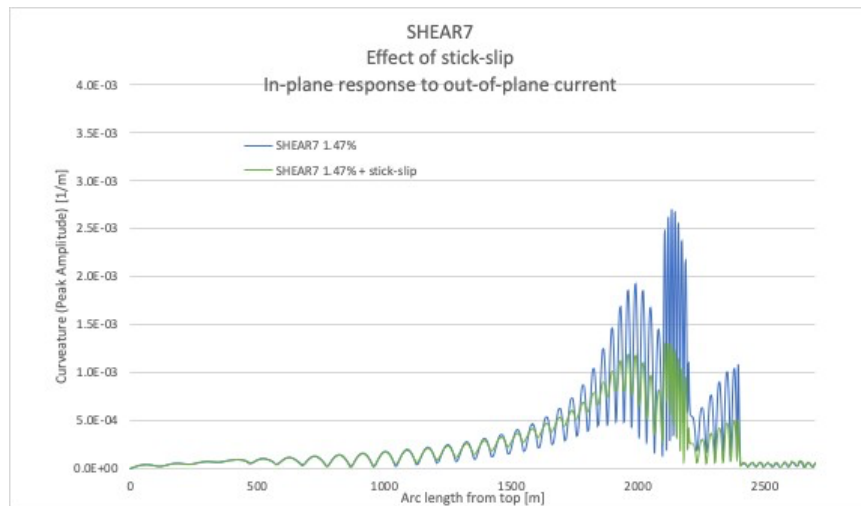
Figure I-5: SHEAR7 predictions on effect of stick-slip on umbilical from OMAE2016-54816
