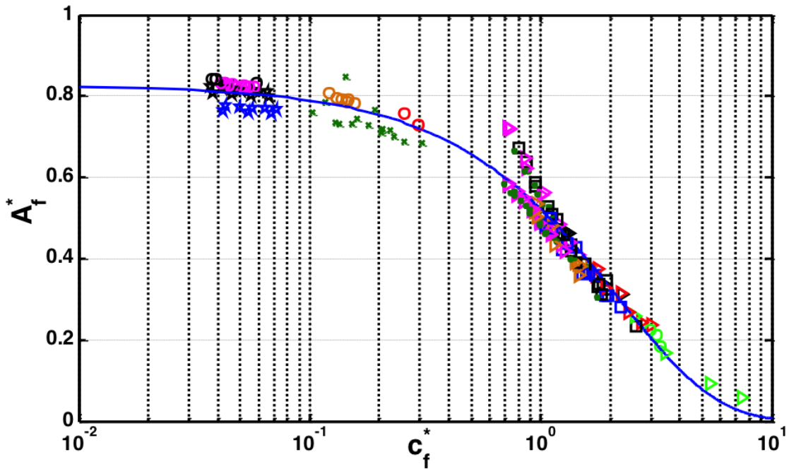
Figure H-2: A_f^* versus c_f^* for a wide range of top tension, SCR and lazy wave risers with and without stakes. The branch on the top side of the curve revealed a program bug during development testing that was subsequently resolved prior to release.
