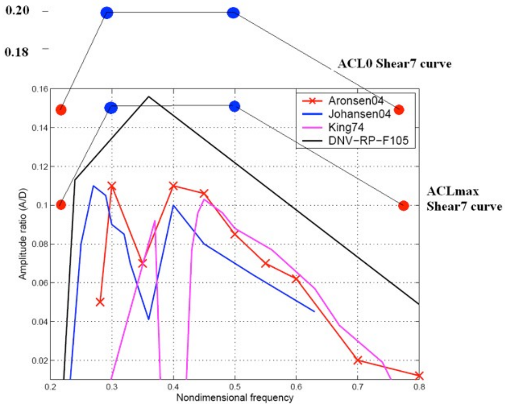
Figure G-1: Summary of A/D at CL = 0 limits from Ref [1], along with limits of common.s7CL curves for common.s7CL Table 7
