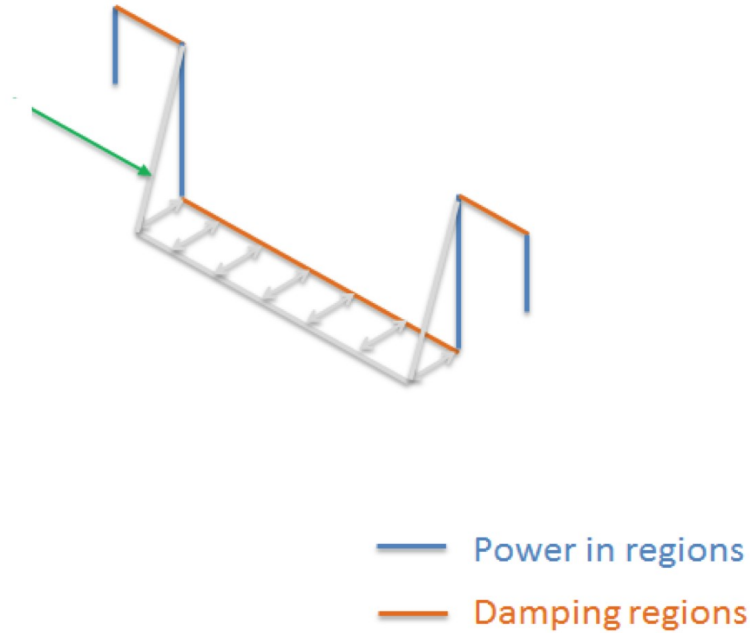
Figure F-1: Jumper schematic highlighting power-in and damping regions when modelling axial flow
