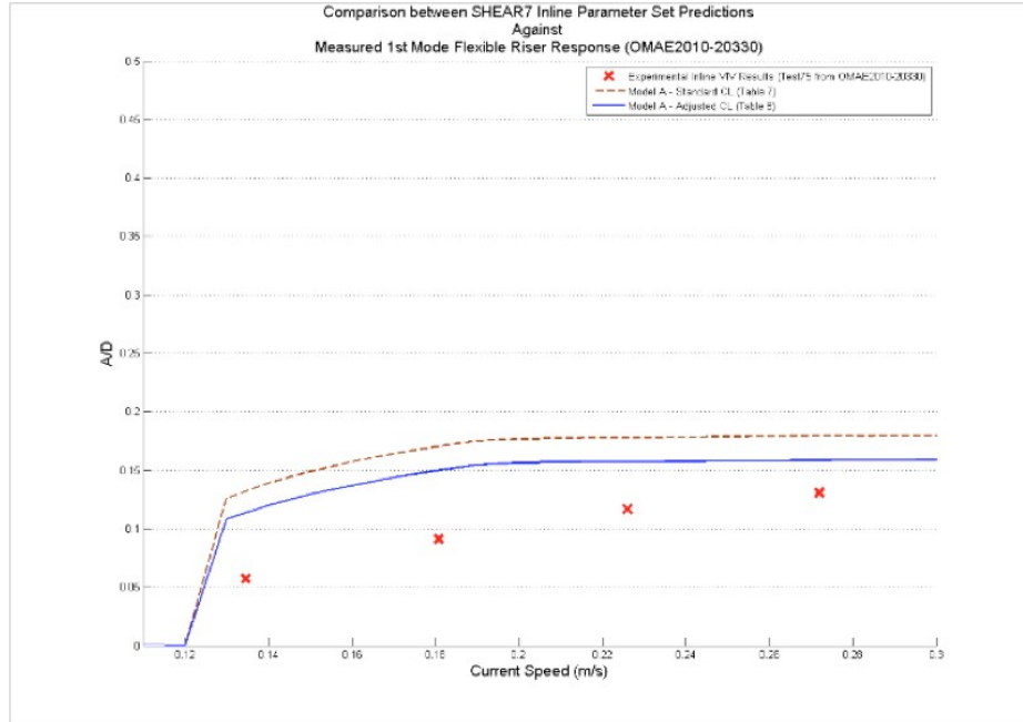
Figure G-3: Comparison between SHEAR7 using common.s7CL Tables 7 & 8 and the Test 75 Series Experimental Results A/D vs Current Velocity
