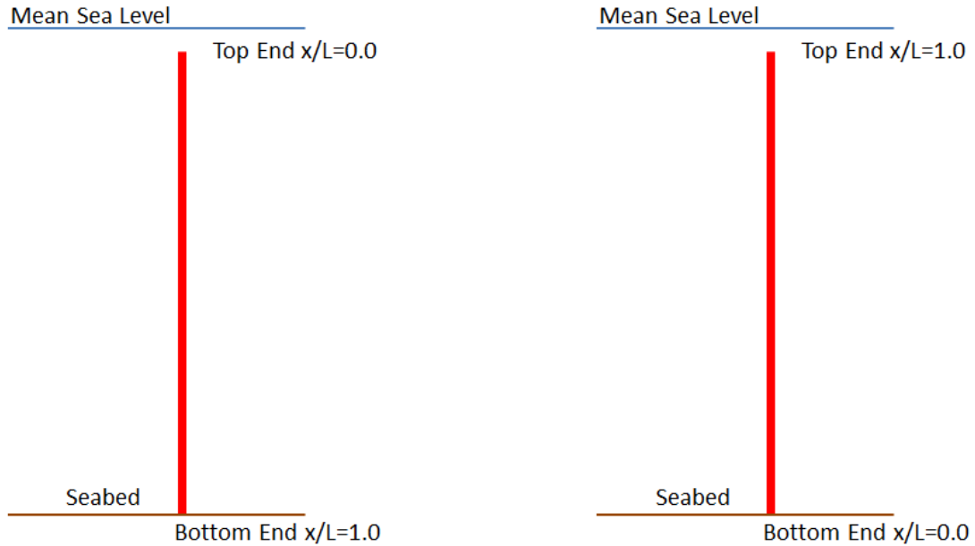
Figure 1: SHEAR7 Coordinate System
