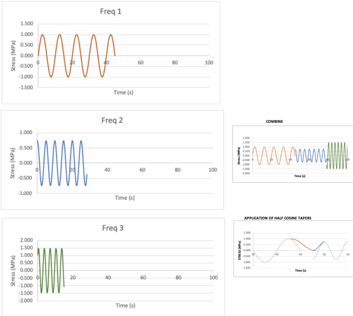
Figure K-1: Illustration of how time sharing is combined for the stress time history
