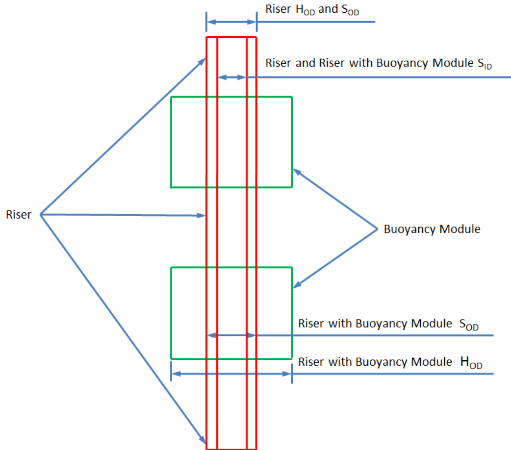
Figure 5: Example of Diameters in a Riser with Buoyancy Module Sections
