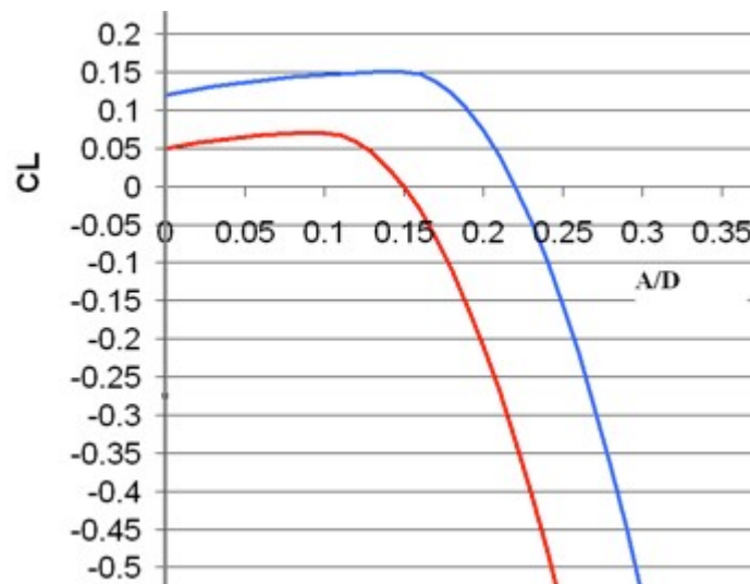
Figure G-2: common.s7CL curves for common.s7CL Table 7
