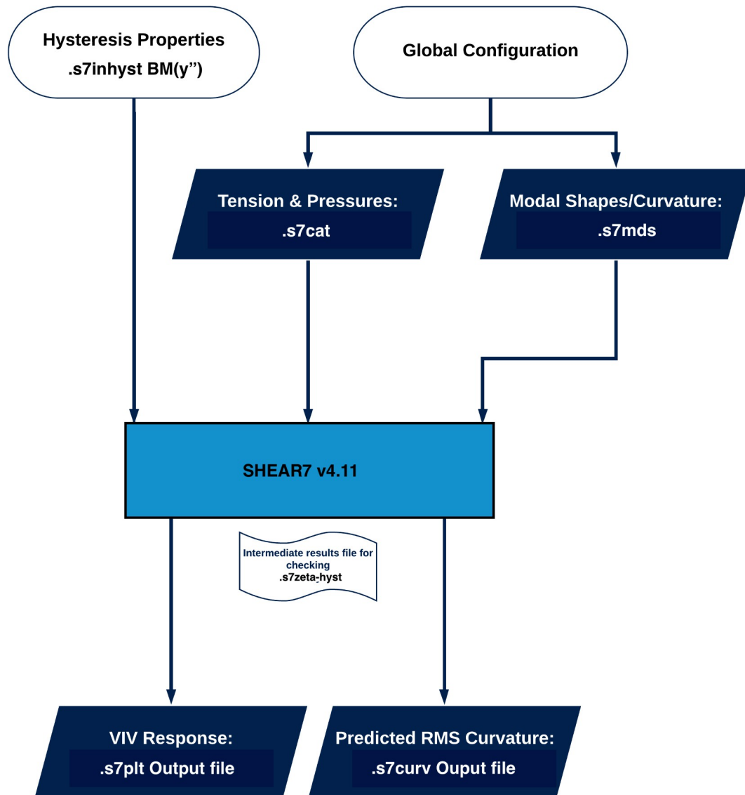
Figure I-1: Inputs/Outputs Summary for Varying Structural Damping Module
